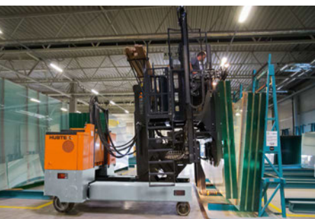
M 90 preparing customer orders
