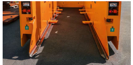
GTR with special device to transport glass stillages with fork pockets
